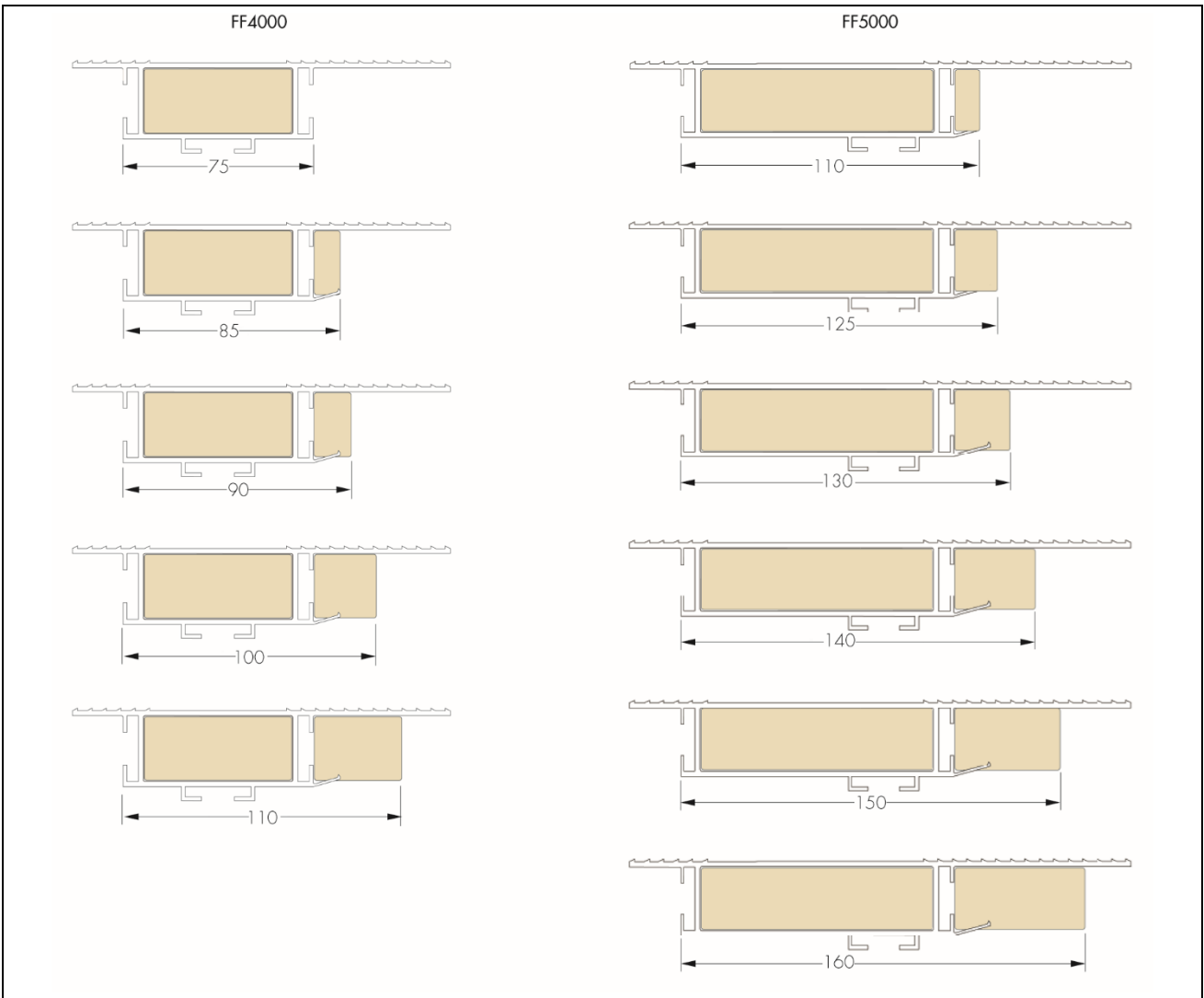
Figure 1 FF4000 and FF5000 closers (all dimensions in mm) (example sizes)
