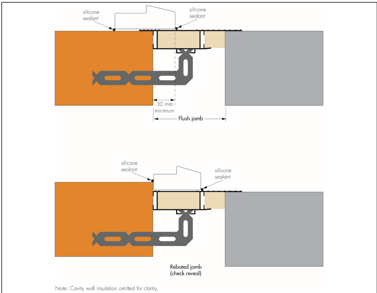
Figure 3 Typical jamb details
